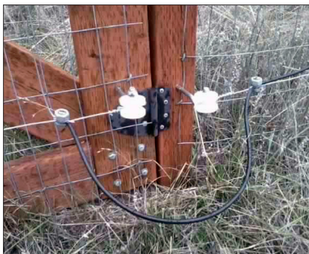
Figure 4. Black-colored insulated electric fence wire, 12-gauge. Used here to connect the electrified lines of a gate to the main electrified lines on the fence.
