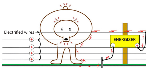
Figure 1. An all-hot electrified fence design. All wires are connected to each other in series and to the positive terminal on the energizer. The negative terminal of the energizer is connected to the grounding rod.
