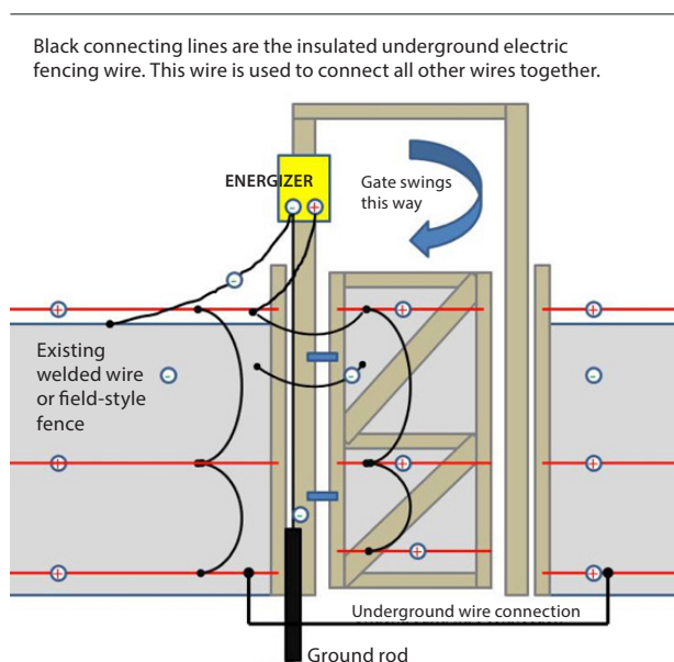
Figure 8. An example of how a gate can be electrified by attaching it to the electrified lines on the main fence, and how two sections of fence can be electrified with an underground wire connection.
