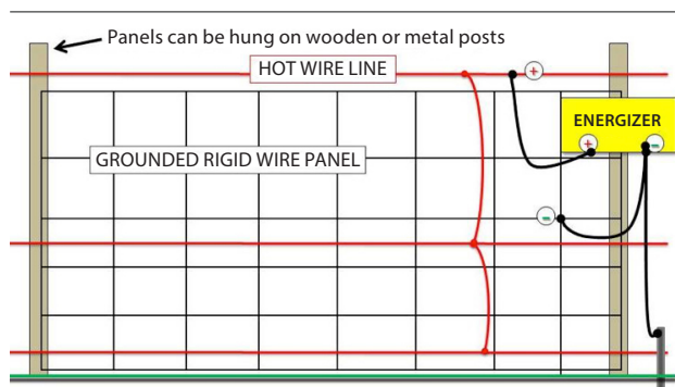
Figure 6. Rigid wire panel or net-wire fencing with three electrified wires attached to the outside of the fence. The electrified wires are connected in a series and attached to the positive terminal of the energizer. Then, panel or net-wire fence is connected to the negative terminal of the energizer. The ground rod is also connected to the negative terminal of the energizer.
