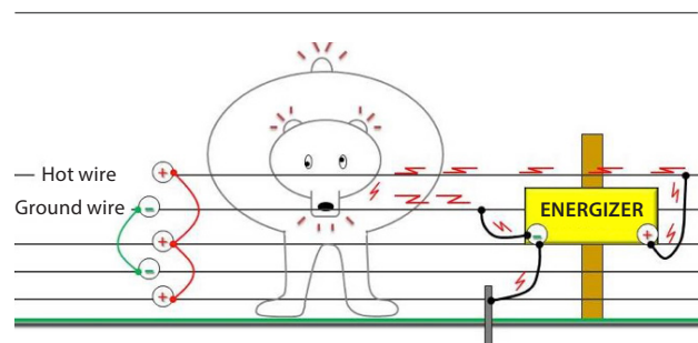
Figure 2. A ground-return electrified fence design. All hot wires are connected to each other in a series and to the positive terminal on the energizer. All ground wires are connected to each other and to the negative terminal on the energizer. The negative terminal of the energizer is also connected to a grounding rod.
