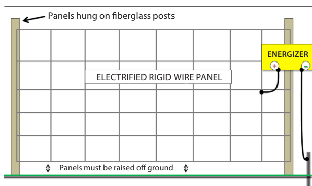
Figure 5. Electrified rigid wire panel. The panel is raised off the ground and insulated by hanging it from fiberglass posts. The wire panel is electrified by connecting it directly to the positive terminal on the energizer. The ground rod is connected to the negative terminal of the energizer.
